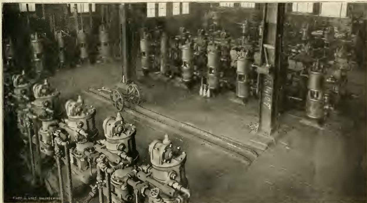
VIEW OF A CORNER IN THE PUMP ROOM OF THE WESTINGHOUSE AIR BRAKE COMPANY'S WORKS, WILMERTON, PA
